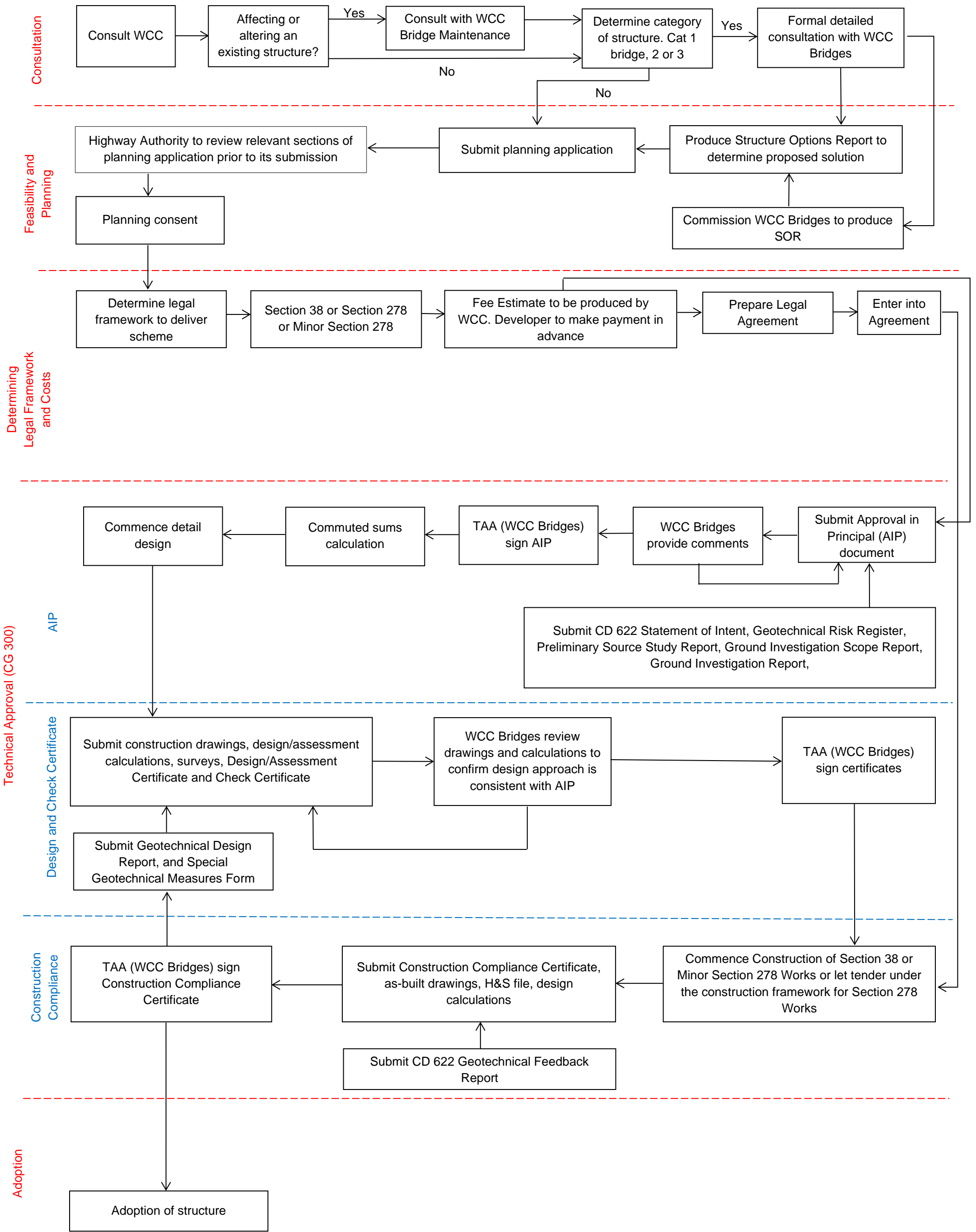
Figure 7.1.1 Process Flowchart
