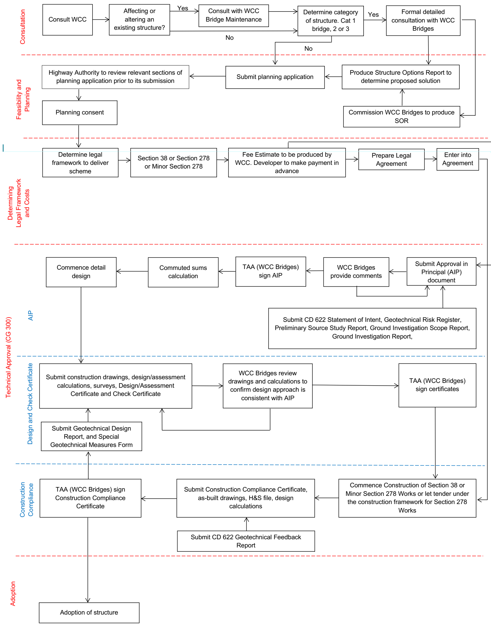
Figure 7.1.1 Process Flowchart
