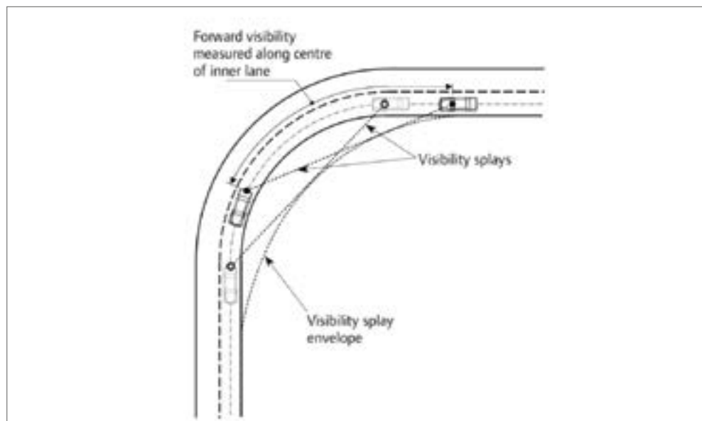
Figure 3.4 - Measurement of Forward Visibility (Reference: MfS Figure 7.19)
