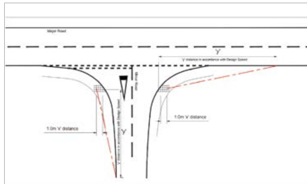
Figure 3.5 - Pedestrian Visibility Splays at Junctions
