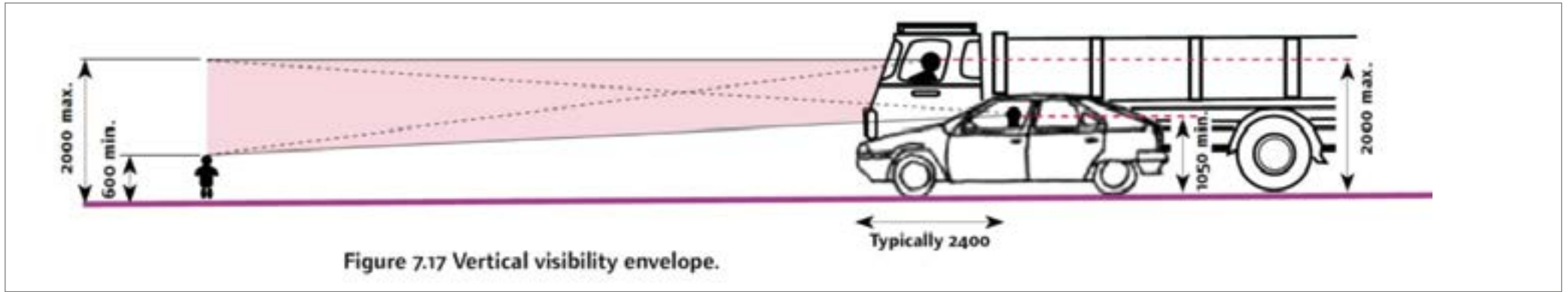
Figure 3.6 - Vertical Visibility Splay (Reference: MfS Figure 7.17)
