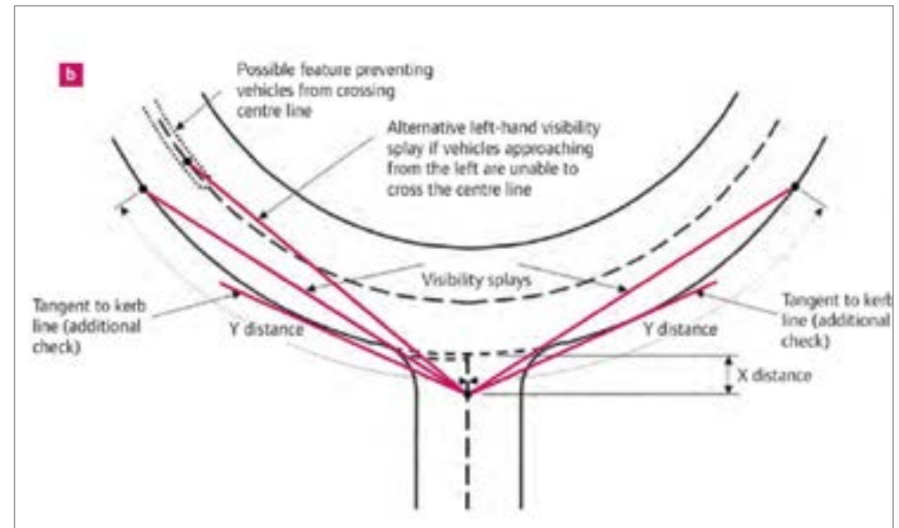
Figure 3.3 - Visibility Splay on Bend (Source: Extract from MfS Figure 7.18)
