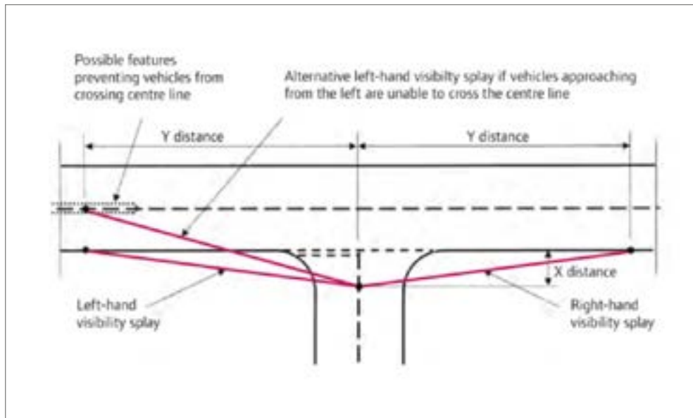
Figure 3.2 - Straight Road Visibility Splays (Extract from MfS Figure 7.18)
